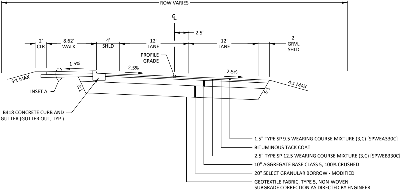
HORNSBY STREET NE PROPOSED TYPICAL SECTION #1 STATION 1+26 TO 6+00
