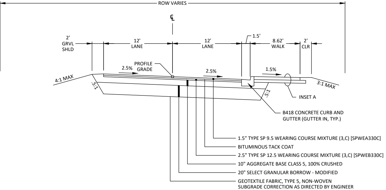
EUREKA AVENUE N PROPOSED TYPICAL SECTION #4 STATION 63+20 TO 65+50
