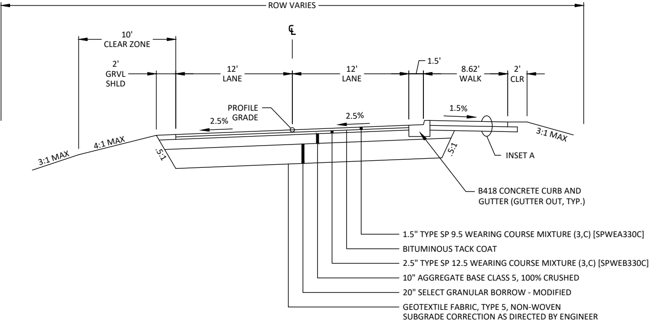
EUREKA AVENUE N PROPOSED TYPICAL SECTION #3 STATION 18+70 TO 62+00 STATION 66+70 TO 70+00
