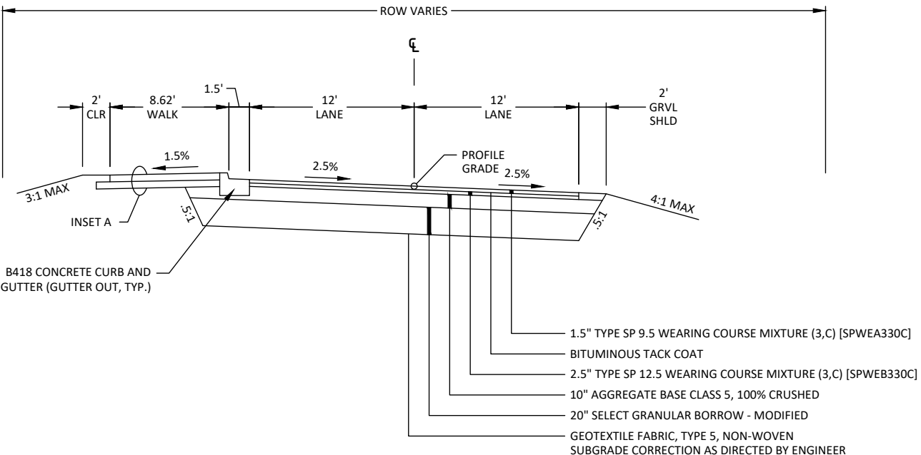
HORNSBY STREET NE / EUREKA AVENUE N PROPOSED TYPICAL SECTION #2 STATION 7+00 TO 17+50
