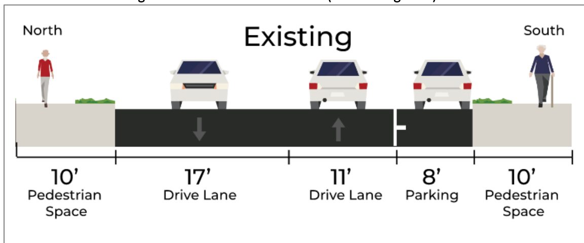
Figure 9: 2 nd Street Cross Section (Proctor Segment)
