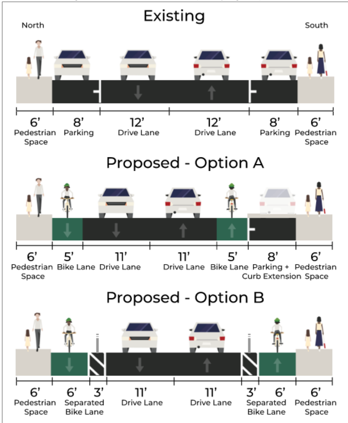
Figure 11: 2 nd Street Cross Section (County Segment)
